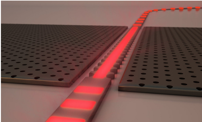
A zero-index waveguide compatible with current silicon photonic technologies. Credit: Second Bay Studios/Harvard SEAS
